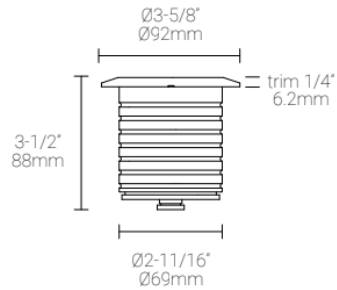
Fixture Detail:
