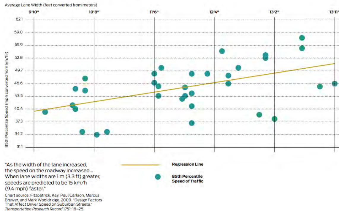
Figure B4. Research findings on lane width and traffic speeds Wider travel lanes are correlated with higher vehicle speeds.
