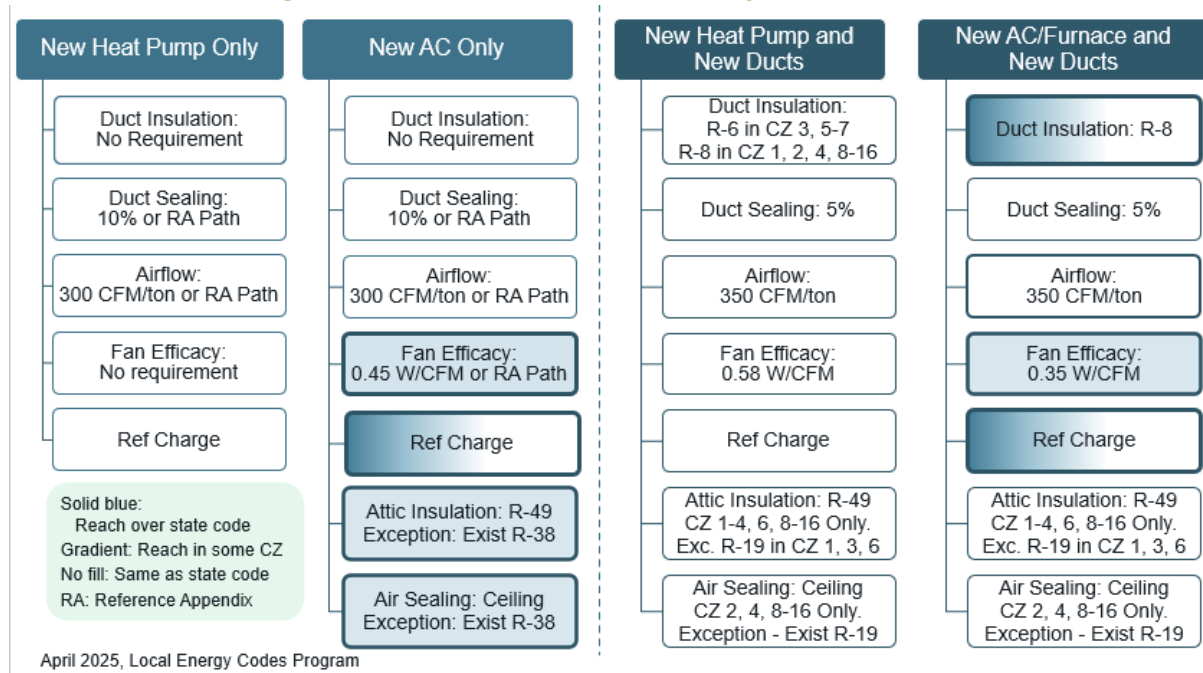
Figure 1. AC vs. Heat Pump Pathway Requirements
