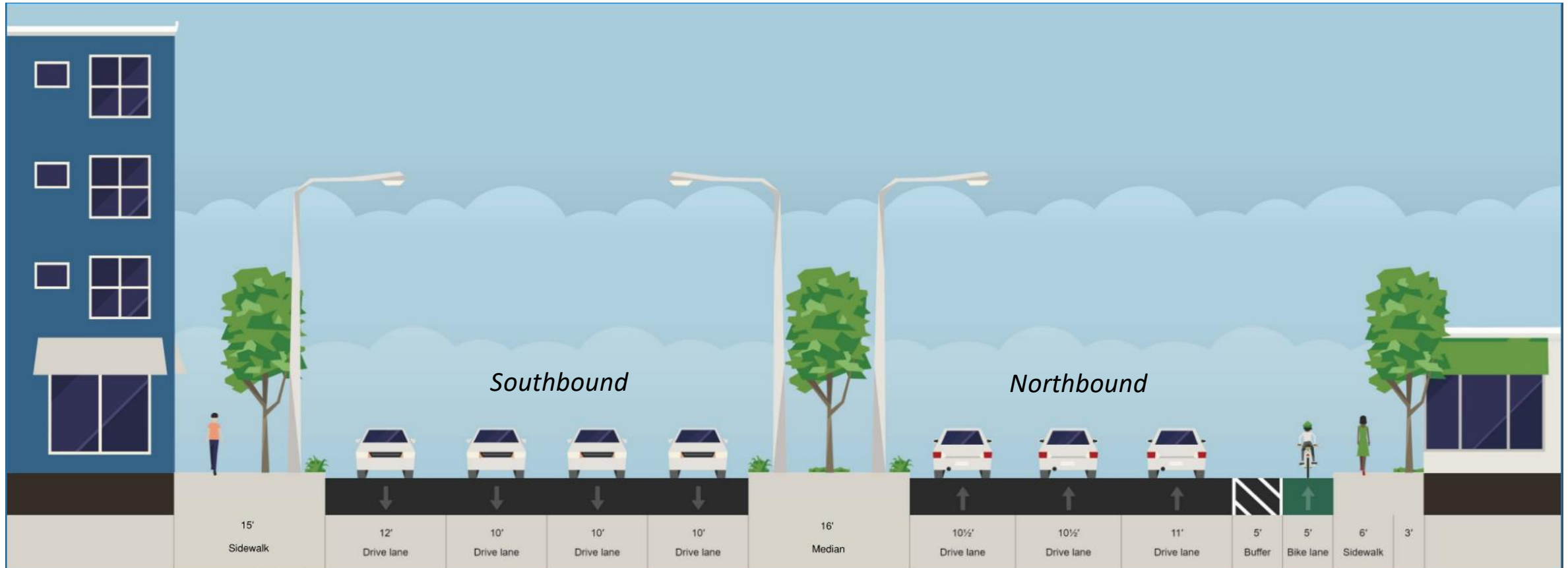
*Typical Cross Section
