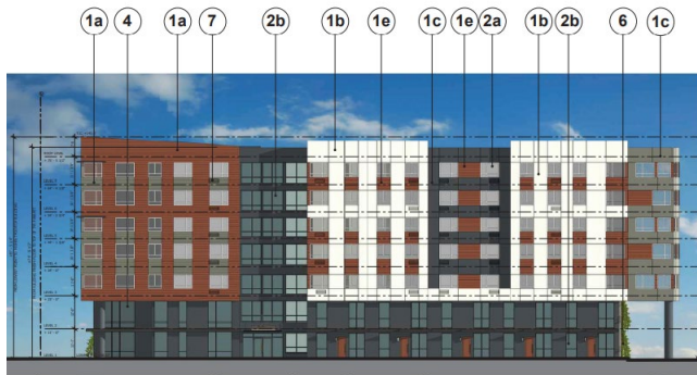
B NORTH ELEVATION SCALE: 1/16"=1'-0"
